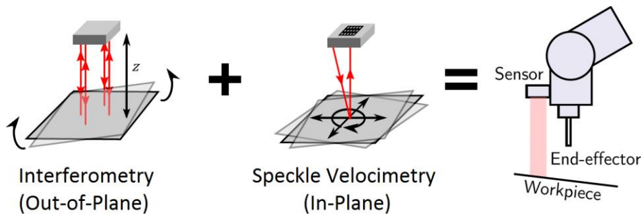
6 degrees of freedom robotic end-effector sensing
