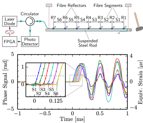
Speed-of-sound measurement using fibre segment interferometry
