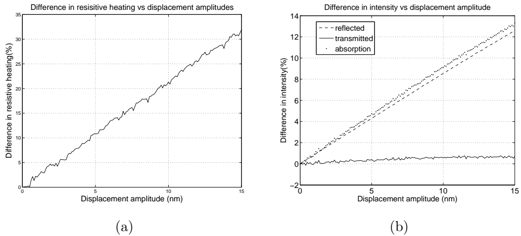
Figure 4.60: (a) The mean time-averaged resistive heating in the d-eCHOT models (extracted from the background film). It can be seen that the resistive heating is increasing with the displacement amplitude, as a percentage of the resistive heating when there is no SAW (when the displacement amplitude is zero). It can be seen that the increase is linear with the displacement amplitude. This demonstrates the contribution of the resistive heating to the device operation (b) The difference in the reflected and the transmitted field intensity of an eCHOT as a percentage of the incident intensity at different displacement amplitudes. The reflected component is essentially twice the signal amplitude, which grows linearly. The transmitted component has a smaller slope. It can be seen that the amount of change in transmission is not big enough to compensate for the increase in the reflected component. This further demonstrates that the absorption/resistive heating is the main operating mechanism in d-eCHOT. Also shown is the calculated absorption from the model. It has a bigger slope than the difference in reflection, since the transmission is out of phase with the absorption.
