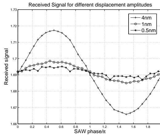
Figure 4.52: The demonstration of the effect of numerical noise on the signal for small displacement amplitudes. The same model with the same number of elements are run for different displacement amplitudes. It can be seen that as the displacement amplitude is reduced, the obtained signal amplitude (reflectivity) decreases and becomes more noisy. In these models, a transducer with 100nm finger thickness and 25nm background film thickness is used. The maximum mesh element size was set to 53nm ( \lambda_o/15 ) while the minimum element size was around 8nm (in the background film).
