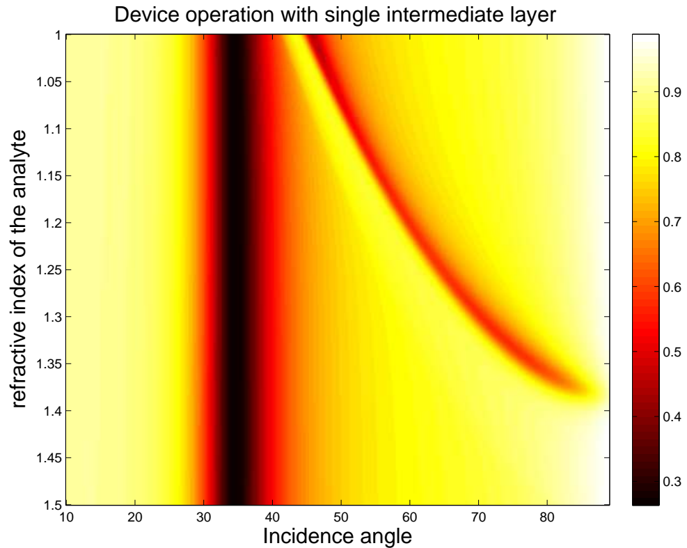
Figure 4.8: The reflectivity at various incidence angles for a simple self-calibrated SP sensor, when the refractive index of air (the subdomain with refractive index n_2 in figure 4.9) changes. The thickness of the intermediate ( MgF_2 ) layer is 200nm. Reflected field is observed at various incidence angles(x-axis), at each value of n_2 (y-axis), which is varied between 1 and 1.5. It can be seen that there is a dip with constant angular location(along x-axis) and a dip that moves along x-axis when the analyte refractive index is varied. This property suggest the use of this structure as a calibrated refractive index sensor.
