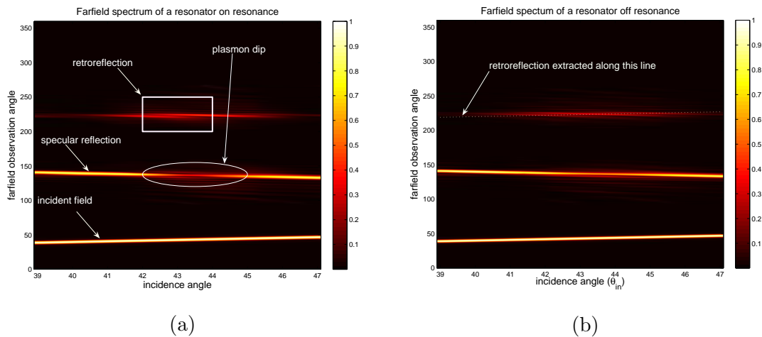
Figure 4.18: The farfield spectrum of the plasmon resonator (normalised with the incident field intensity). The retroreflection can be seen between farfield angles 220^\circ - 225^\circ when the incidence angle is 40^\circ - 45^\circ (refer to figure 4.15 for the explanation of the conventions for the farfield angles). (a) The resonator is on resonance. The dip in the specular reflection is low, and the retroreflection is high compared to (b) . Also the SPR dip is wider than the SPR dip on flat films. This broadening is due to the width of the cavity on which plasmons can be excited. (b) The farfield spectrum of the resonator close to off-resonance. It can be seen that retroreflection is lower than (a) and the dip in the specular reflection is not as deep. The rising of the dip value shows the destructive interference of the launched plasmons with the reflected ones. Also shown is the dotted lines corresponding to the retroreflection.
