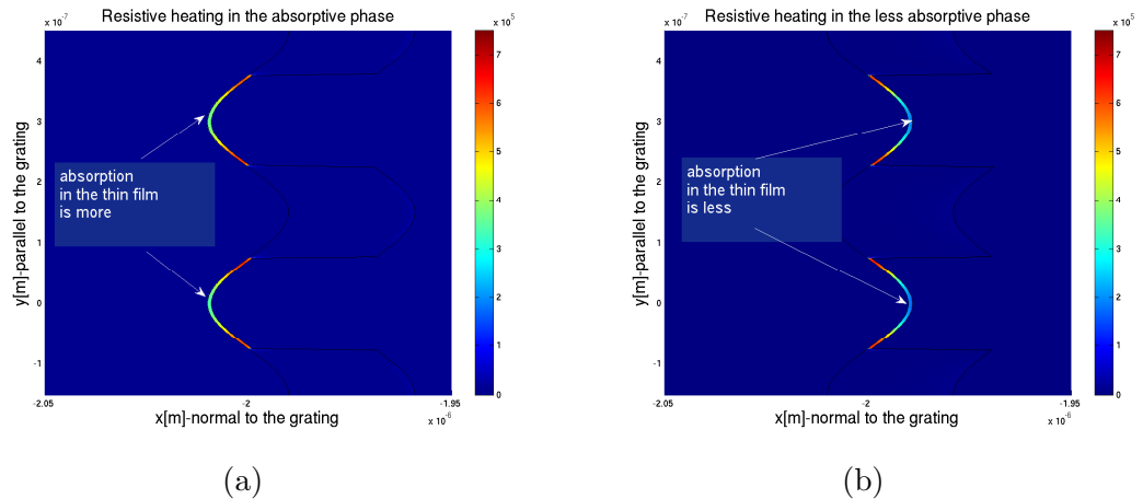
Figure 4.49: The demonstration of the modulation of the absorption in the thin film in eCHOT. (a) Resistive heating in the thin film in the absorptive phase. (When the phase of the SAW is such that the thin film moves into an evanescent field increasing the absorption.) (b) Resistive heating in the thin film, in the less absorptive phase. (When the phase of the SAW is such that the thin film is moved out of the evanescent field yielding less absorption)
