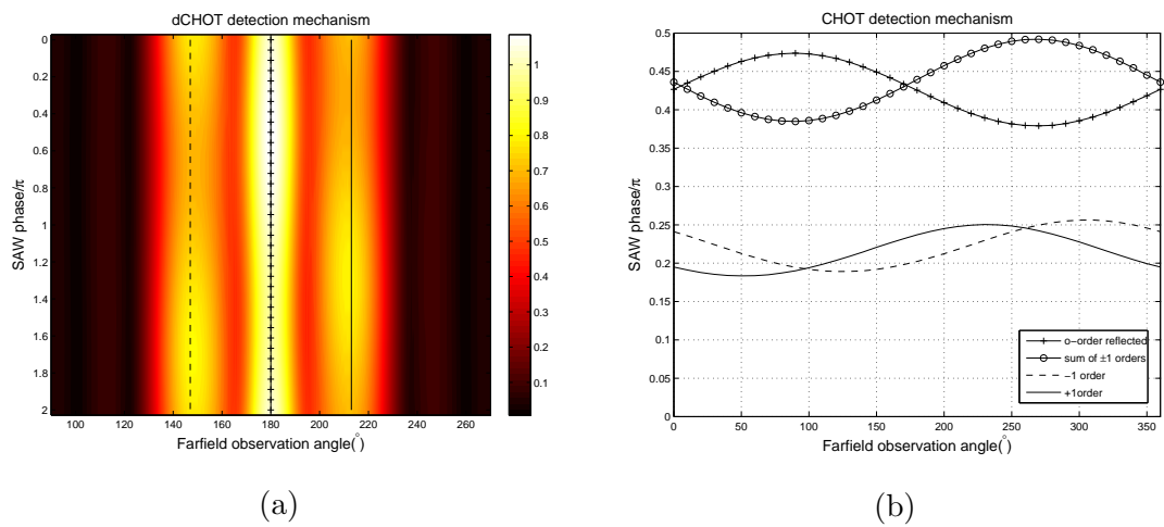
Figure 4.46: The operation characteristics of the d-CHOT. (a) The reflected farfield spectrum of the d-CHOT mechanism. The diffracted orders are seen at farfield observation angles, 147^\circ and 213^\circ . The 0-order reflection is also seen at 180^\circ (b) The intensity of different propagating components vs the SAW phase. This plot shows what happens to the intensity of the different field components as the SAW interacts with the d-CHOT. None of the diffracted orders are individually 180^\circ out of phase with the 0-order reflected, however, their sum is completely out of phase with the 0-order reflected field, which suggests that the lost intensity in the 0-order reflection is compensated equally by the diffracted orders.
