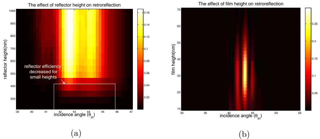
Figure 4.30: (a) The effect of the reflector height in the resonator efficiency. As can be seen, for small reflector heights there is less retroreflection. This is due to the fact that SPs can go over such small obstacles. (b) The effect of metal film thickness in the resonator efficiency. Film thickness directly related to the coupling to plasmons. The optimal film thickness was found to be around 30nm for silver for \lambda_{in} = 639nm
